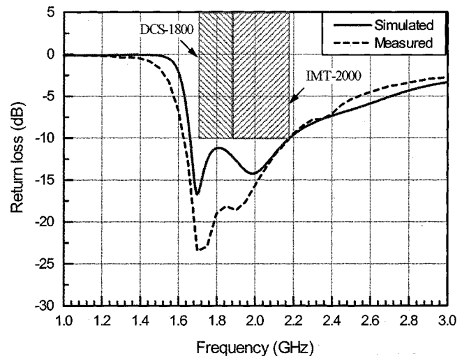
Fig. 2. Simulated and measured return loss.
