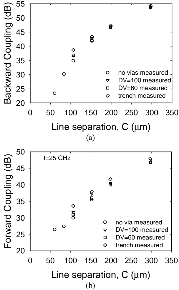
Figure 5: Measured (a) backward coupling and (b) forward coupling of microstrip lines fabricated on different layers of polyimide (Figure 1b) as a function of center to center spacing, C.
