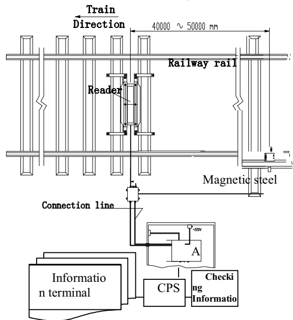
Fig.3 Components of ATIS
