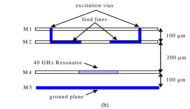
Fig. 2 Side view of (a) 60GHz slotted patch resonator (b) 39 GHz slotted patch resonator
