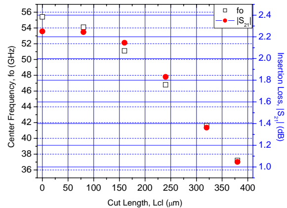
Fig. 4 Simulated responses of center frequency ( f_0 ) and insertion loss ( |S_{21}| ) as a function of transverse cut ( L_{cl} )
