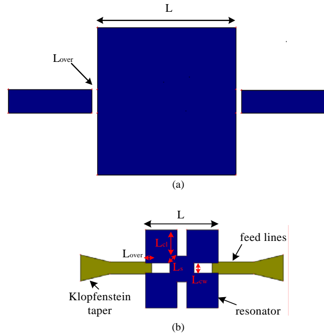
Fig. 1 Top view of (a) conventional \lambda/2 square patch (b) Miniaturized patch resonator.
