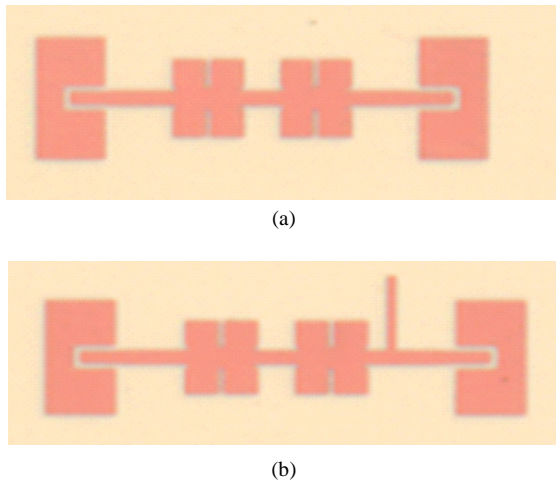
Fig. 7 Photograph of the fabricated millimetre-wave LCP band pass filter with (a) two resonators (b) two resonators and a rejection stub
