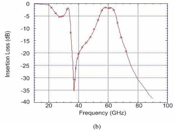
Fig. 8 Measured insertion loss with (a) two resonators (b) two resonators and a rejection stub
