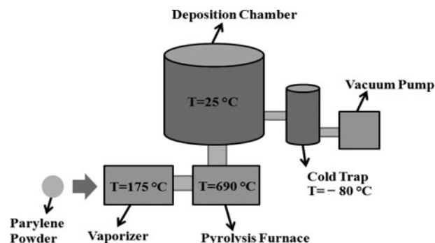
Fig. 2. General Parylene deposition system.
