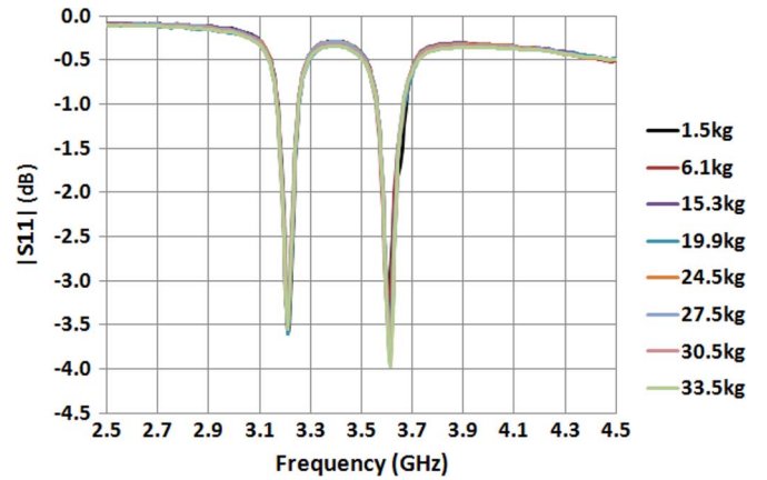
Fig. 18. Measured |S_{11}| of the fabricated prototype with y -polarization excitation subjected to various attached weights.
