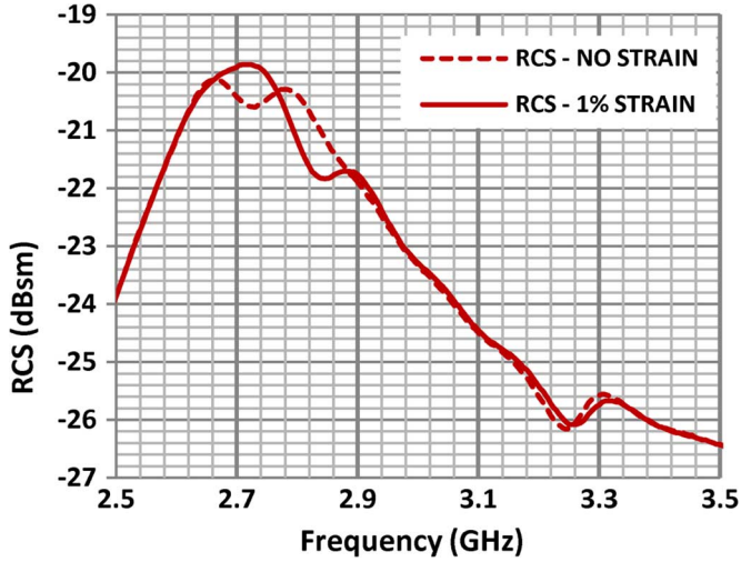
Fig. 23. RCS responses due to the loading effect of the strain transducer (without impedance transformer).
