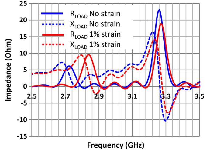
Fig. 22. Input impedance Z_{LOAD} of the patch-loop strain sensor when no strain (blue lines in online version) and 1% strain (red lines in online version) are applied.
