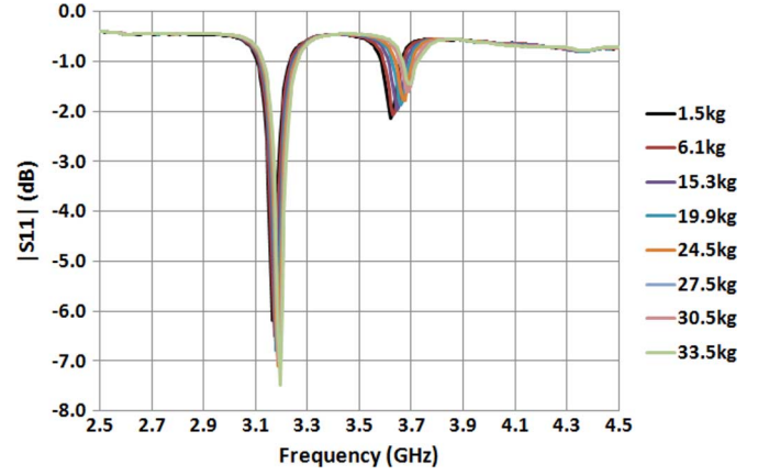
Fig. 17. Measured |S_{11}| of the fabricated prototype with x -polarization excitation subjected to various attached weights.
