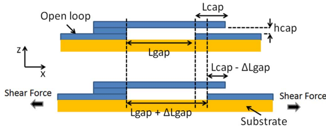
Fig. 4. Cross-section view of a cantilever implemented on a modified loop loaded in the new strain sensor.
