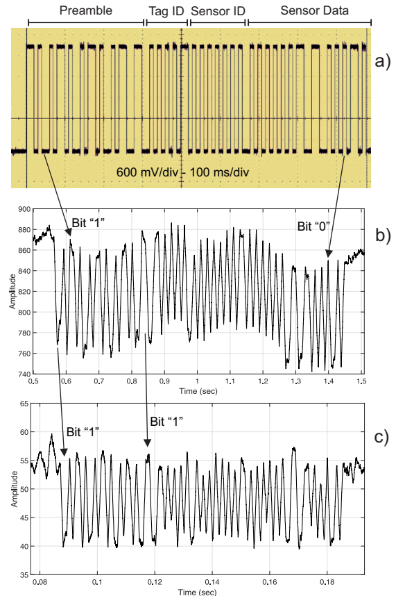
Fig. 5. Time domain backscatter packet signals, (a) oscilloscope measurement of transmitted rectangular pulses, (b) received packet pulses at T_{\text{symbol}} = 10 ms, (c) received packet pulses at T_{\text{symbol}} = 1 ms.
