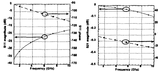
Fig. 5b. Extracted \mu BGA S-parameters.
