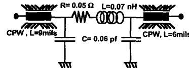
Fig. 5a. Extracted \mu BGA hybrid model
