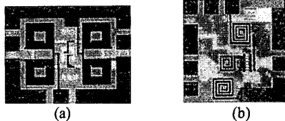
(a) (b) Fig. 11. Photo of the Tx chipset used in the module (a) Mixer (b) RF amplifier
