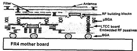
Fig. 1. 3D integrated module concept view.
