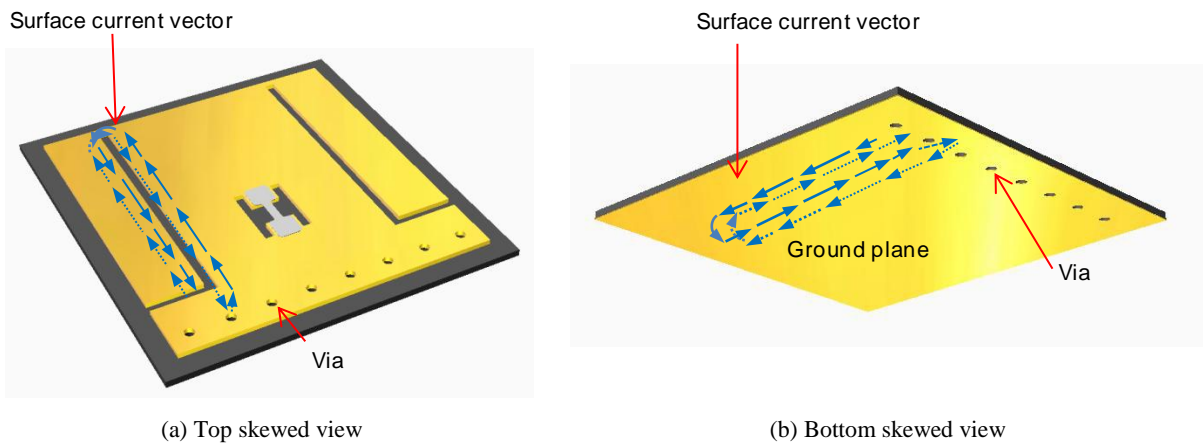
Fig. 6. Illustration of the surface current vector in the slotted patch antenna (dotted lines represent current on the opposite surface of the view).
