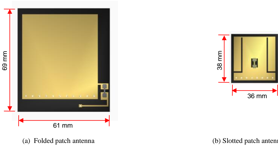
Fig. 5. Footprint comparison of the folded patch antenna sensor and slotted patch antenna sensor
