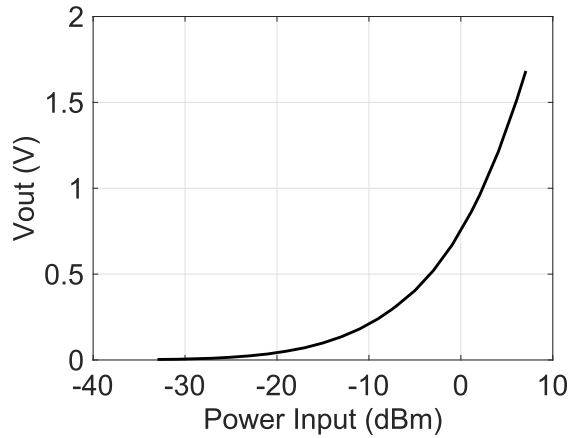
Fig. 7. Measured output voltage of “double” converter across the 1588- \Omega load. The two input signals have the same phase at the frequency of 2.4 GHz.
