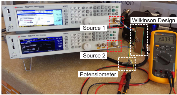
Fig. 10. Two signal generators measurement setup. The one generator has a fixed zero-phase 2.4-GHz signal. The second generator was used for the phase sweeping.
