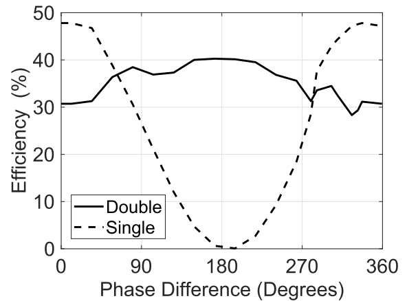
Fig. 13. Measured converter efficiency versus phase difference at the input. The input signals had a frequency of 2.4 GHz with P_{in} = 8 dBm.
