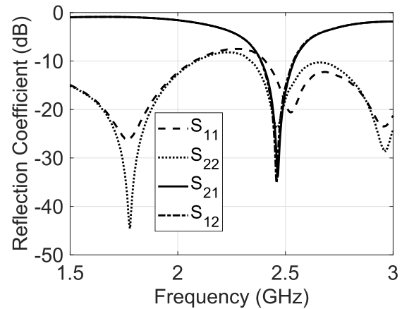
Fig. 5. S-parameters of “double” design. The VNA available input power ( P_{in,i} ) at each port was fixed at -20 dBm.
