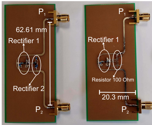
Fig. 3. Two fabricated designs on the low-cost FR-4 substrate. Left: “double” design includes two rectifiers. Right: “single” design includes one rectifier and one isolation resistor.
