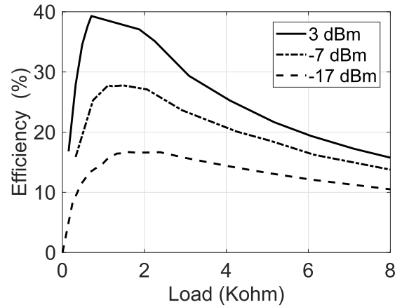
Fig. 8. Measured “double” rectifier efficiency versus load for a different available input power at 2.4 GHz.
