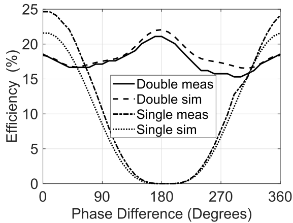
Fig. 11. Simulated and measured converter efficiency versus phase difference at the input. The input signals had a frequency of 2.4 GHz with P_{in} = -17 dBm.
