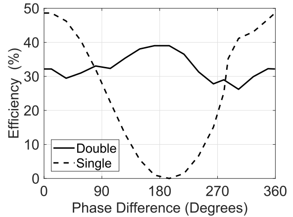
Fig. 12. Measured converter efficiency versus phase difference at the input. The input signals had a frequency of 2.4 GHz with P_{in} = 3 dBm.
