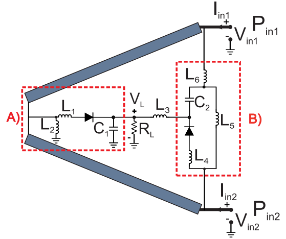
Fig. 2. Circuit of the double design. Two single rectifiers (dash rectangle) have been combined using a common load R_L .
