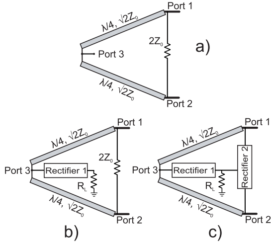
Fig. 1. Power combiner circuits with rectification capabilities. (a) Typical Wilkinson combiner circuit. (b) Wilkinson combiner circuit with a single rectifier. (c) Wilkinson combiner with two rectifier circuits. One rectifier has been installed at port 3, and the isolation resistor has been replaced with the second rectifier.
