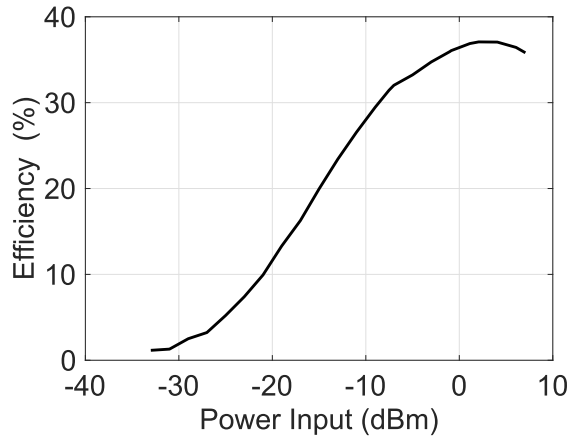
Fig. 6. Measurement rectifier efficiency of “double” design versus the available input power ( P_{in} ). The two input signals have the same phase at the frequency of 2.4 GHz.
