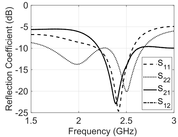
Fig. 4. S-parameters of “single” design. The VNA available input power ( P_{in,i} ) at each port was fixed at -20 dBm.
