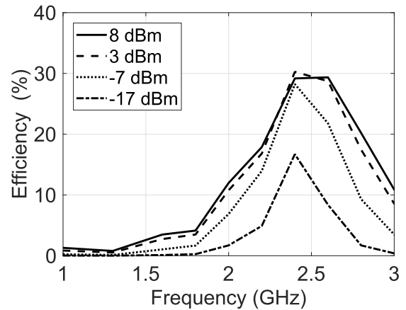
Fig. 9. Measured “double” rectifier efficiency versus frequency for different power input levels. Load is fixed at 1559 \Omega .
